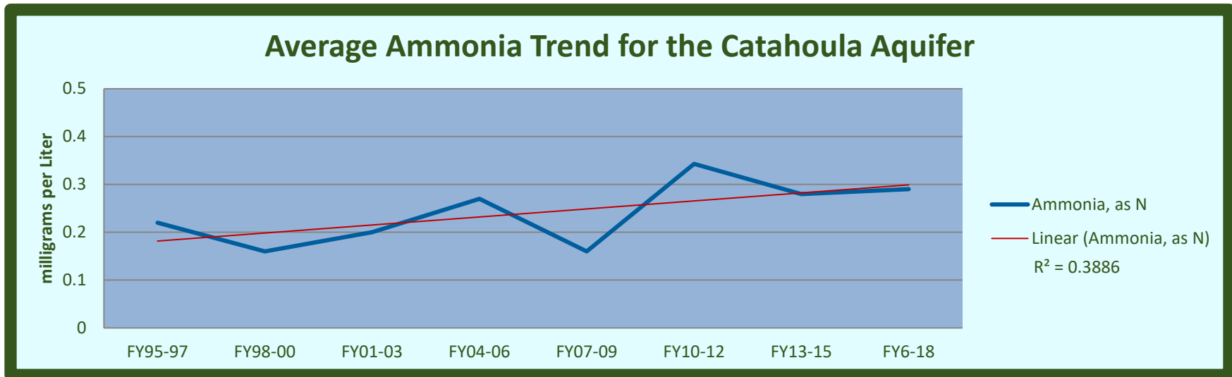
Chart 5-11: Ammonia Trend
