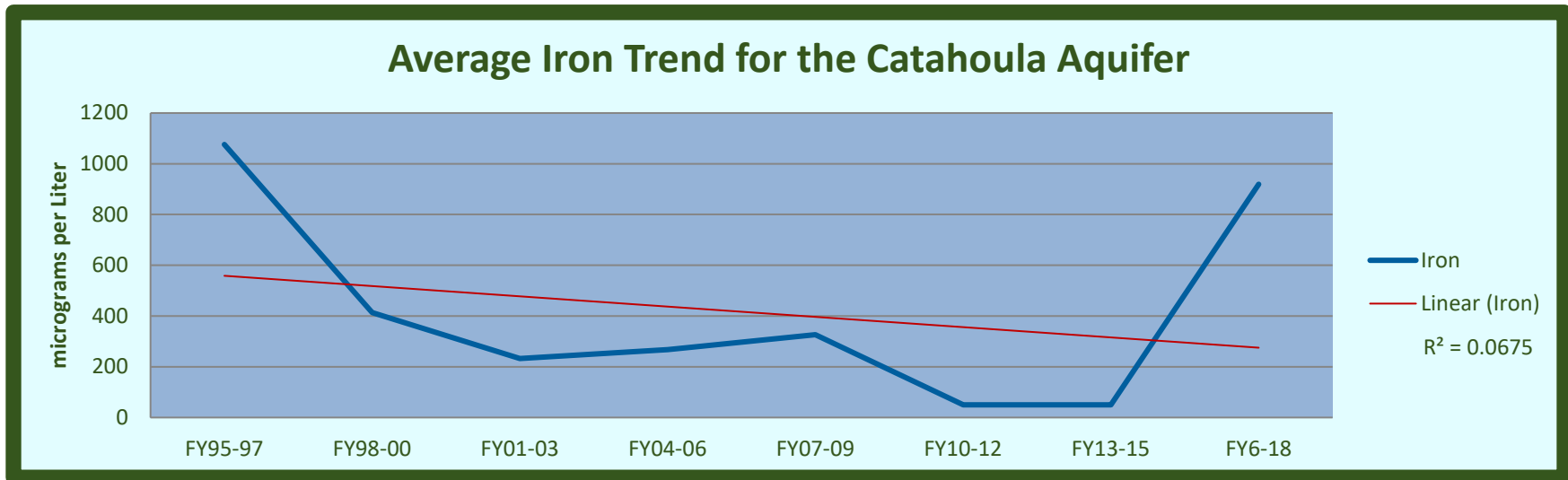
Chart 5-17: Iron Trend
