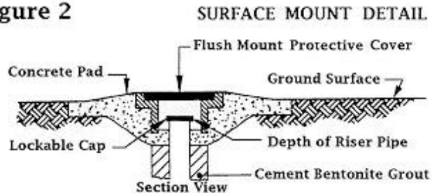
GROUNDWATER MONITORING WELL (TYPICAL) (Not to Scale)
